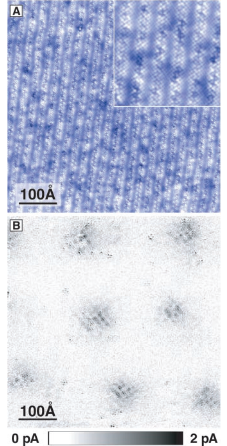
Fig. 1. Topographic and spectroscopic images of the same area of a Bi-2212 surface. (A) A topographic image of the 560 Å field of view (FOV) in which the vortex studies were carried out. The supermodulation can be seen clearly along with some effects of electronic inhomogeneity. The Cu–O–Cu bonds are oriented at 45° to the supermodulation. Atomic resolution is evident throughout, and the inset shows a 140 Å square FOV at \times 2 magnification to make this easier to see. The mean Bi–Bi distance apparent here is a_0 = 3.83 Å and is identical to the mean Cu–Cu distance in the CuO plane \sim 5 Å below. (B) A map of S_1^{12}(x, y, 5) showing the additional LDOS induced by the seven vortices. Each vortex is apparent as a checkerboard at 45° to the page orientation. Not all are identical, most likely because of the effects of electronic inhomogeneity. The units of S_1^{12}(x, y, 5) are picoamps because it represents \Sigma dI/dV \cdot \Delta V . In this energy range, the maximum integrated LDOS at a vortex is \sim 3 pA, as compared with the zero field integrated LDOS of \sim 1 pA. The latter is subtracted from the former to give a maximum contrast of \sim 2 pA. We also note that the integrated differential conductance between 0 and -200 meV is 200 pA because all measurements reported in this paper were obtained at a junction resistance of 1 gigaohm set at a bias voltage of -200 mV.
