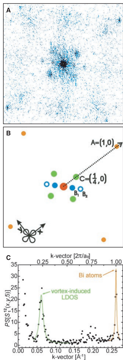
Fig. 2. Fourier transform analysis of vortex-induced LDOS. (A) PS[S_1^2(x, y, 5)] , the two-dimensional power spectrum of the S_1^2(5, x, y) map shown in Fig. 1B. The four points near the edges of the figure are the k -space locations of the square Bi lattice. The vortex effects surround the \mathbf{k} = 0 point at the center of the figure. (B) A schematic of the PS[S_1^2(x, y, 5)] shown in (A). Distances are measured in units of 2\pi/a_0 . Peaks due to the atoms at (0, \pm 1) and (\pm 1, 0) are labeled A. Peaks due to the supermodulation are observed at B_1 and B_2 . The four peaks at C occur only in a magnetic field and represent the vortex-induced effects at k -space locations (0, \pm 1/4) and (\pm 1/4, 0) . (C) A trace of PS[S_1^2(x, y, 5)] along the dashed line in (B). The strength of the peak due to vortex-induced states is demonstrated, as is its location in the k -space unit cell relative to the atomic locations. The spectrum along the line toward (0, 1) is equivalent, but there is less spectral weight in the peak in PS[S_1^2(x, y, 5)] at (0, 1/4) .
