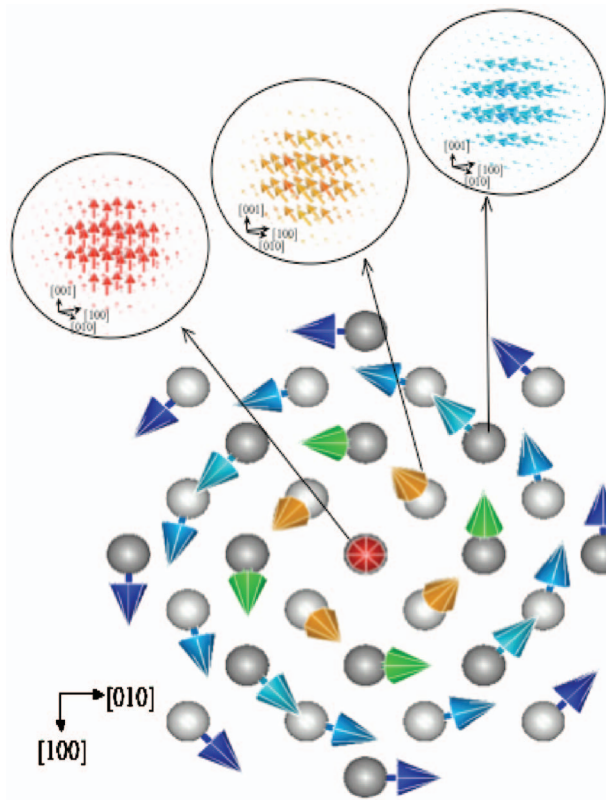
FIG. 8. (Color) Virtual fab representation of the geometry, spin arrangement, and spin densities (insets) of 29 Fe atoms, from electronic structural calculations of Nakamura et al. (2003) carried out via the local-density approximation. The outer shells of Fe atoms have their spin structures constrained to form a magnetic vortex, while the spins of the inner Fe atoms are self-consistently calculated to relax into the vortex structure indicated, with the spin of the central Fe atom forming the out-of-plane singularity, and the spins on the next shell of Fe atoms forming a canted structure.
