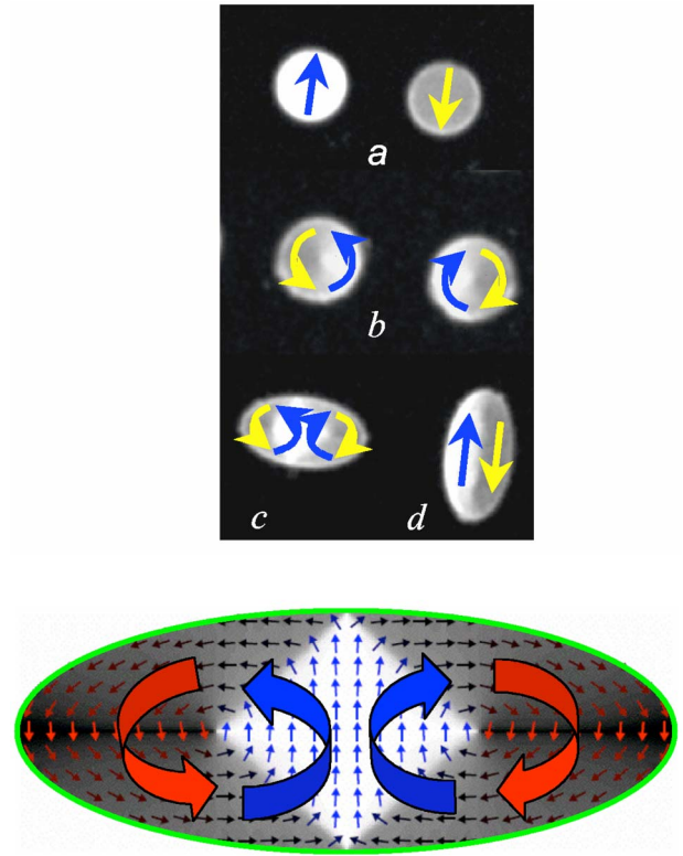
FIG. 9. (Color online) A composite of magnetic images of lithographically patterned Permalloy structures is shown that exhibits size-dependent, metastable remanent states, taken from the work of Buchanan et al. (2005). The images are obtained utilizing the magnetic contrast from resonant x-ray magnetic circular dichroism (XMCD) experiments that utilize photoemission electron microscopy (PEEM) at the Advanced Light Source at Lawrence Berkeley National Laboratory. The samples are subjected to rapidly pulsed magnetic fields and are then imaged in zero field. (a) Two images of single domain states of opposite orientation (with light and dark magnetic contrast, respectively), and (b) two images whose magnetic contrast is indicative of magnetic vortex states of opposite chirality, as indicated by the arrows. The corresponding vortex simulation is shown in Fig. 1(b). (c) The dark-light-dark contrast indicative of a double-vortex spin configuration, as indicated by the arrows and the micromagnetic simulation in the bottom panel, and (d) two opposing magnetic domains that run along the major axis of an elliptically shaped structure. The bottom panel provides a micromagnetic simulation of a double-vortex spin configuration to compare to the image in (c).
