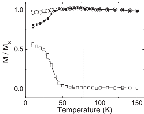
FIG. 4. Normalized in plane longitudinal (solid squares), transverse (empty squares), and total (empty circles) magnetization of \text{FeF}_2(50 \text{ nm})/\text{Ni}(21 \text{ nm}) measured by vector SQUID magnetometry in thermal cycling with a 0.2 T magnetic field. T_N is marked by the dashed line.
