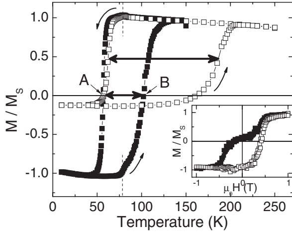
FIG. 1. Normalized magnetization of FeF 2 (50 nm)/Ni(3 nm) measured under temperature sweep in 0.1 T (solid squares) and 0.01 T (empty squares) by SQUID magnetometry. The dashed line marks T_N = 78 K of FeF 2 . The width \Delta T_C is marked by thick horizontal arrows at \langle M \rangle . Points A and B are the reversal temperatures 57 K and 104 K for \mu_0 H_{FC} = 0.1 T (see Fig. 3 for more details). (Inset) Magnetization hysteresis loops for FeF 2 /Ni at T = 10 K for \mu_0 H_{FC} = 0.01 T (solid squares) and 0.1 T (empty squares).
