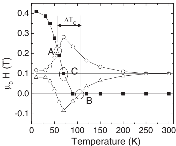
FIG. 3. Exchange bias H_{\text{EB}} (solid squares), H_{\text{FC}} + H_C (empty circles), H_{\text{FC}} - H_C (empty triangles) as functions of temperature. The cooling field H_{\text{FC}} is marked by the horizontal line at 0.1 T. Points A and B mark the reversal temperatures with FM anisotropy considered, in agreement with the position of points A and B in Fig. 1. Point C refers to the reversal temperature for a negligible FM reversal barrier.
