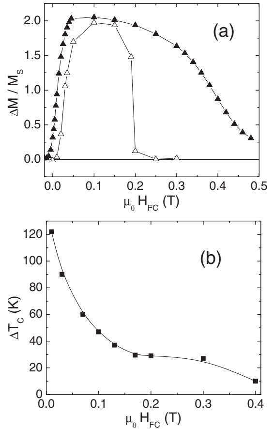
FIG. 2. (a) Magnetic cooling field dependence of the magnetization change \Delta M during fast thermal cycling normalized by the saturation magnetization M_S for FeF 2 /Ni (solid triangles) and FeF 2 /Co (open triangles). A cooling speed dependence results in systematic and controllable differences of up to 10% in \Delta M . (b) Magnetic field dependence of the full thermal width \Delta T_C at \langle M \rangle . Lines are guides to the eye.
