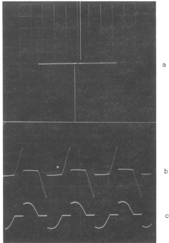
FIG. 1. Response of switching unit to 60-Hz voltage. (a) I - V characteristic: vertical, 2 mA/div; horizontal, 5 V/div. (b) Voltage: vertical, 5 V/div; horizontal, 5 msec/div. (c) Current: vertical, 20 mA/div; horizontal, 5 msec/div.
