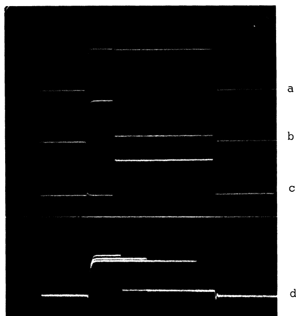
FIG. 2. Response of switching unit to square-wave pulse. Horizontal time scale 500 nsec/div. (a) Voltage applied across unit and 1000- \Omega series resistor: vertical, 5 V/div. (b) Voltage across unit: vertical, 5 V/div. (c) Current through unit: vertical, 10 mA/div. (d) Same as (b) for different amplitudes of applied voltage pulse.
